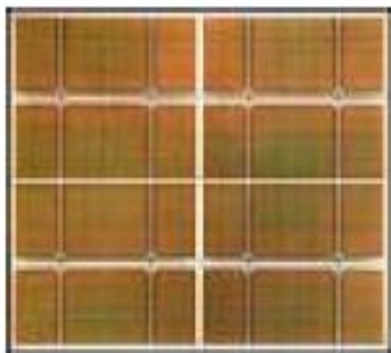
4GB DRAM (2001)
