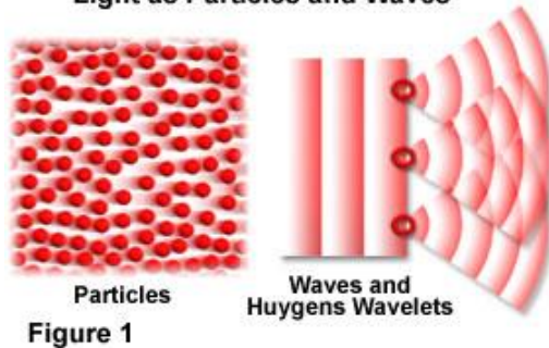
Light as Particles and Waves
