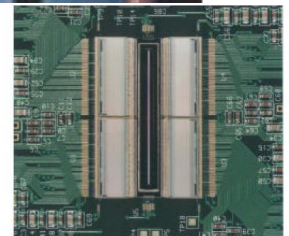
Multi-chip module consisting of four custom driver dies and a 1,080 element linear GLV array.
