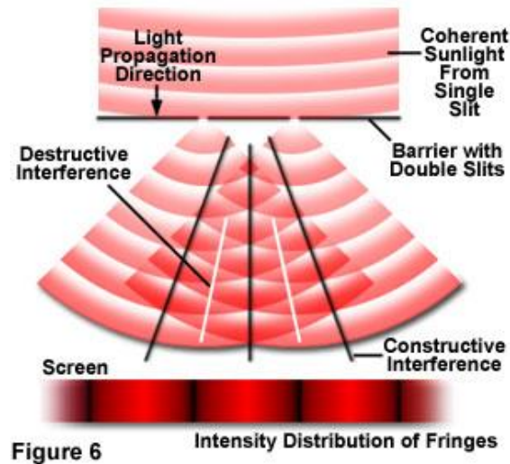
Young's Double Slit Experiment
