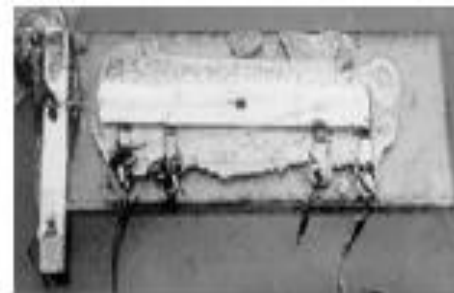
First IC by Kilby
