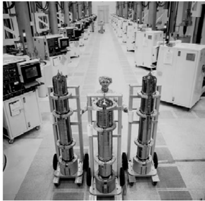
Left: Silicon crystal ingots grown by the Czochralski crystal drawers in the background
