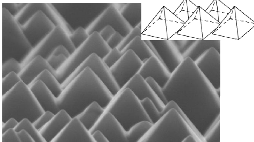
Scanning electron microscope photograph of a textured silicon surface
